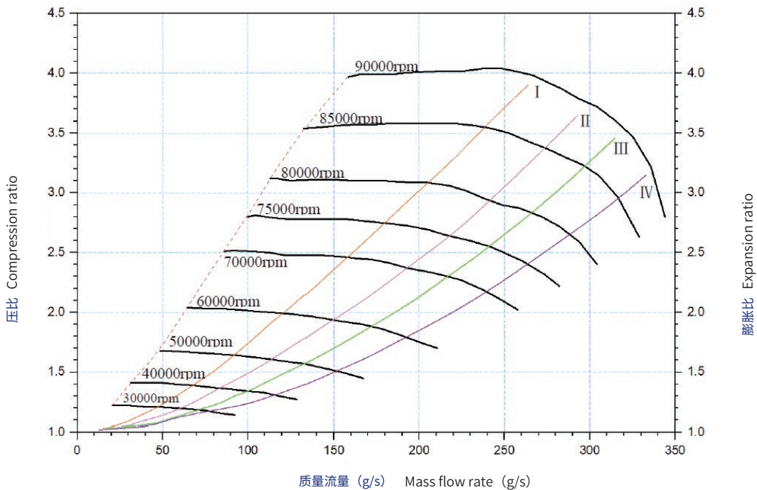
压缩系统特性图 Compression system characteristics chart
