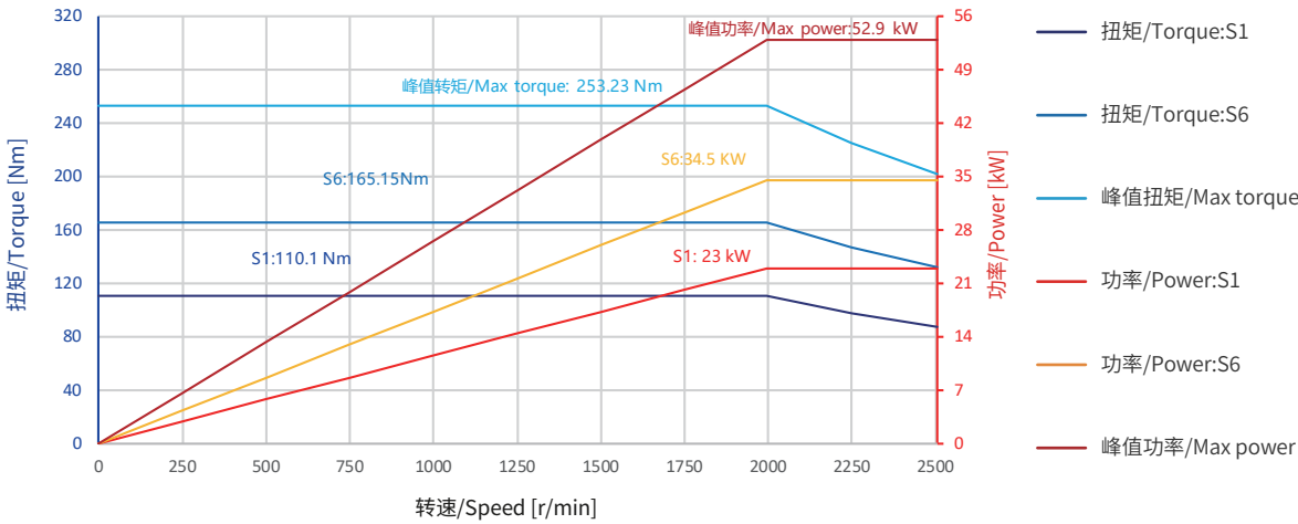
电机特性曲线图 Motor characteristic curve
