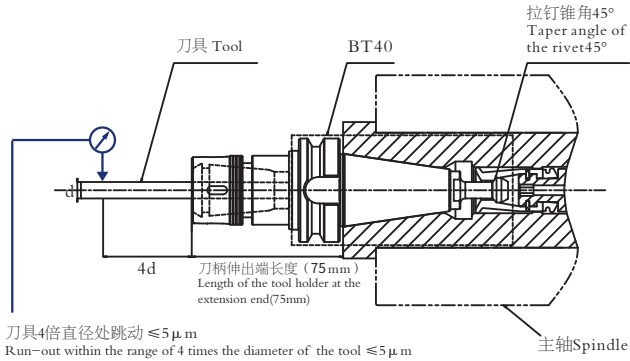
DBT40-45-DKR11-075 (装刀精度示意图 Tool installation precision diagram)
