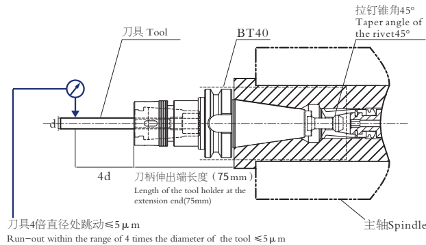
DBT40-45-DSK11-075 (装刀精度示意图 Tool installation precision diagram)
