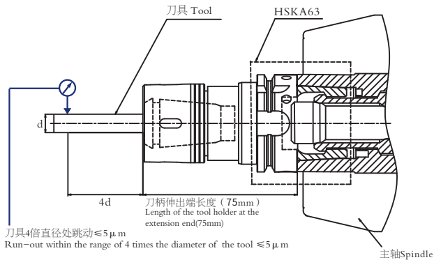
DHSCA63-DKR11-075 (装刀精度示意图 Tool installation precision diagram)
