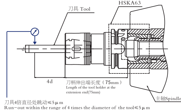
DHKA63-DER11-075 (装刀精度示意图 Tool installation precision diagram)
