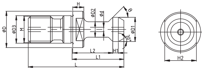
(图1:中心冷却适用Applicable to center cooling)
